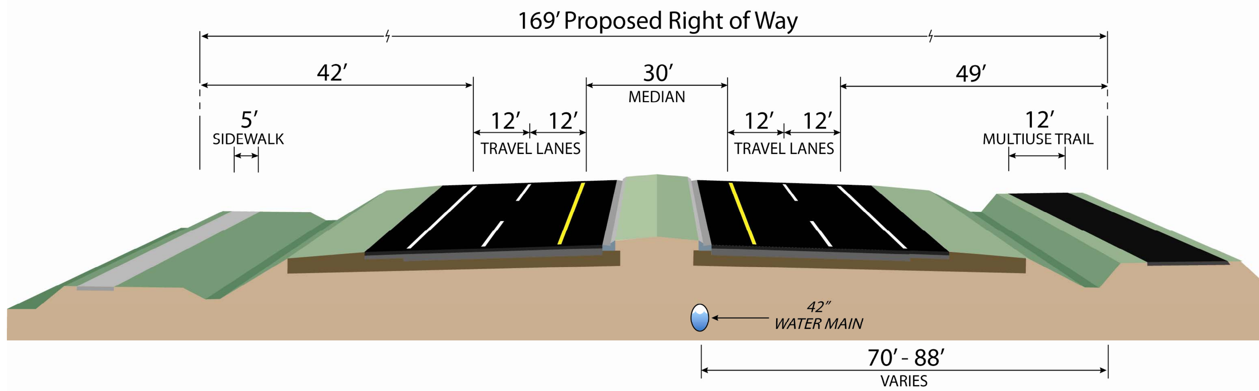
SUBURBAN TYPICAL SECTION 55 mph Design Speed
