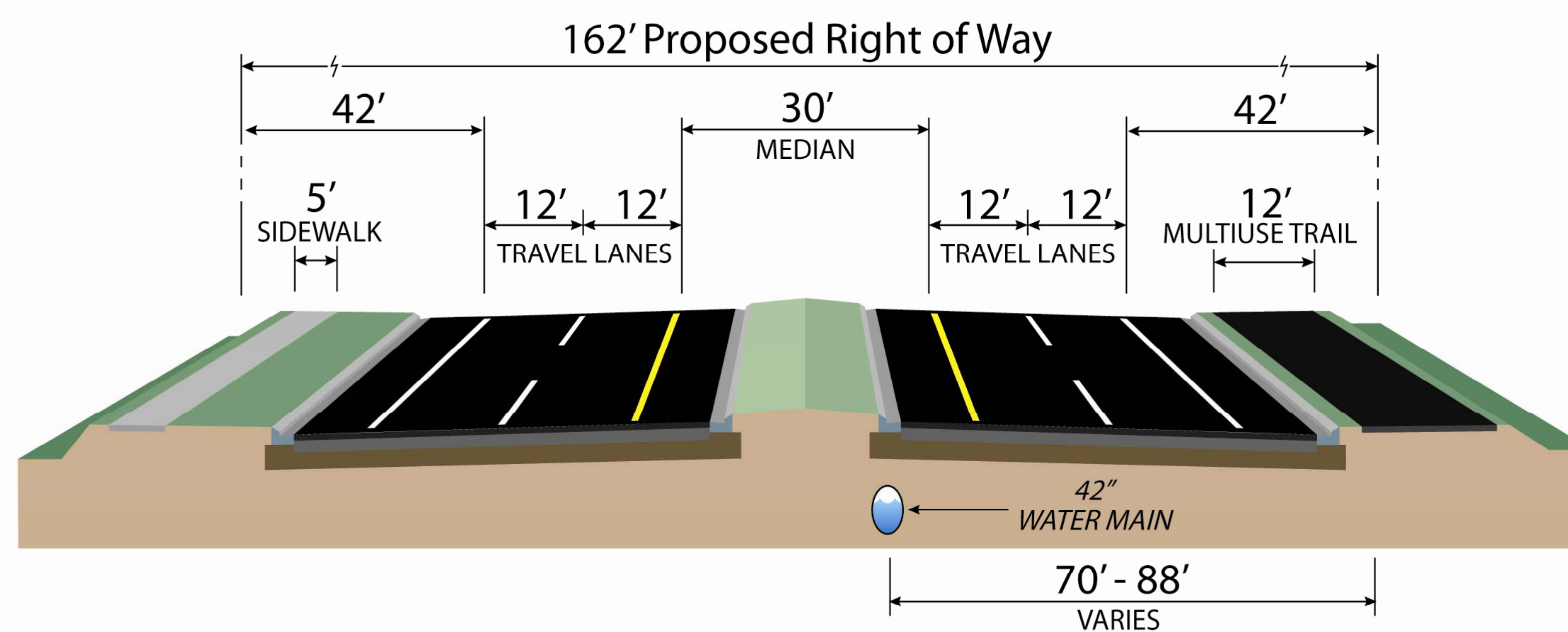
HIGH SPEED URBAN TYPICAL SECTION 55 mph Design Speed
